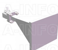
LB-34-20-C-KFSPO Standard Gain Horn Antenna 22-33GHz 20dB Gain 2.92mm Female
