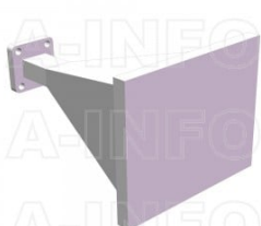
LB-34-20-ASPO Standard Gain Horn Antenna 22-33GHz 20dB Gain Rectangular Waveguide Interface
